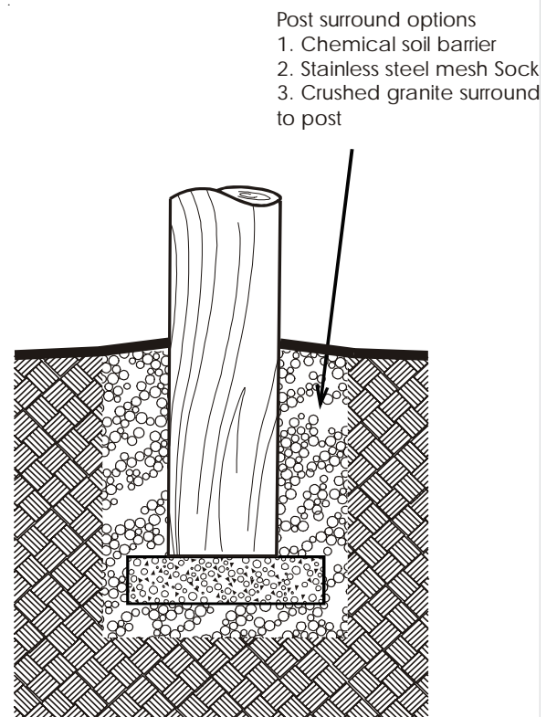
(c) Post surround options (AS 3360.1)
